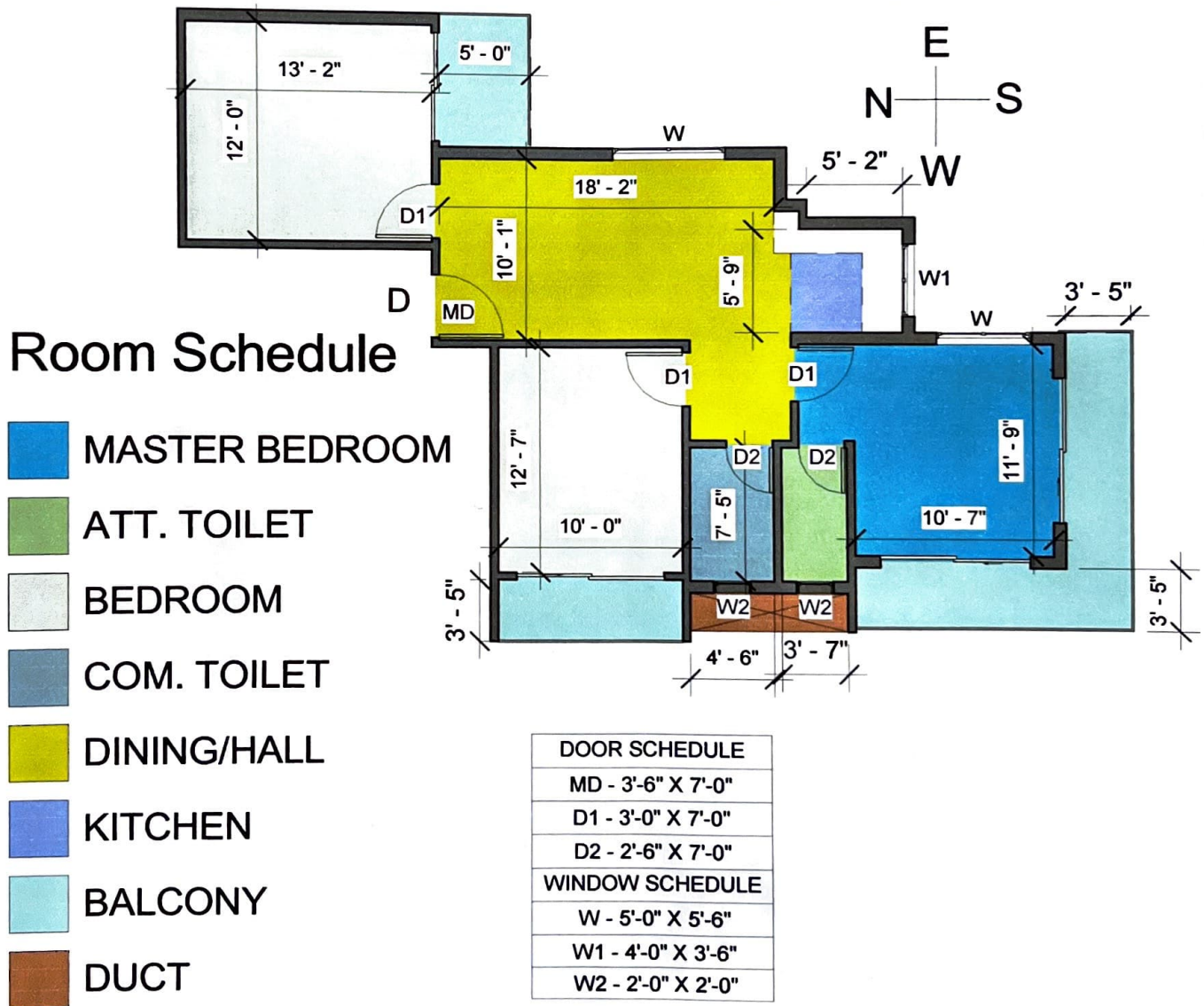
2ND,4TH FLOOR PLAN - D TYPE
